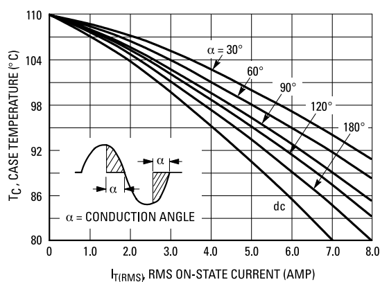
Figure 1. Current Derating
